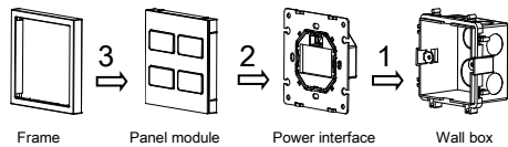
Figure 5. Installation
