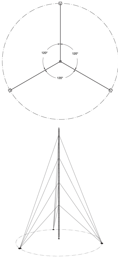
Turret base foundation ground plate (Central node) and guy wires foundation ground plates (intermediate/external node).
