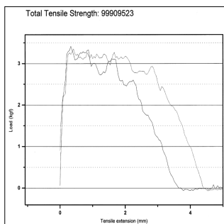
Total pull strength exceeds 3 kg before it disconnects
