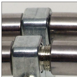
The new CX3 Spring Connect™ keeps continuity and remains RF tight until it's completely disconnected.
