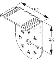
SG 4988 Bracket
