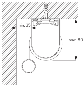
Installation profile SG 10534 and clamp SG 3044
