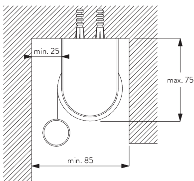
Brackets SG 10873
