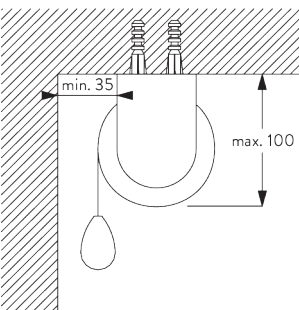
Brackets
