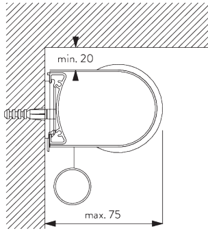
Installation profile SG 10534, brackets SG 1198 and click bracket SG 10539
