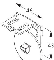
SG 11198 Bracket
