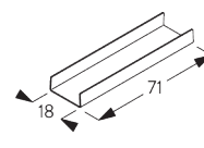
SG 3256 Cover
