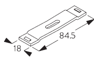
SG 3115 Bracket
