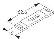
SG 3113 Bracket
