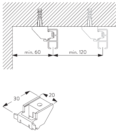
SG 3603 Bracket
