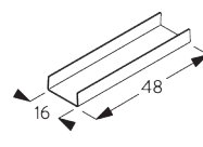
SG 3255 Cover
