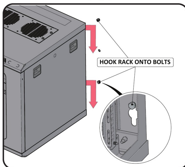
4. Hook Rack onto Bolts
