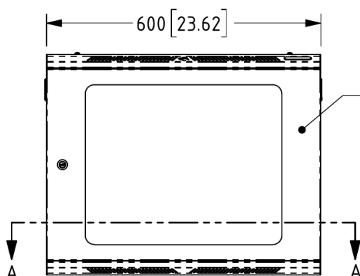
REMOVEABLE/REVERSABLE DOOR WITH KEY LOCK PLAIN, POLYCARBONATE OR VENTED
