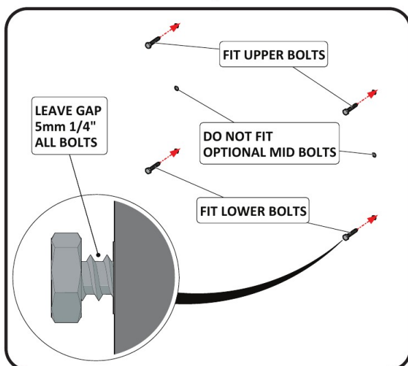
3. Partially Insert Upper and Lower Bolts
