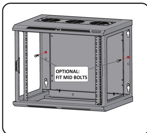
6. Optionally Fit Mid Bolts for Added Security
