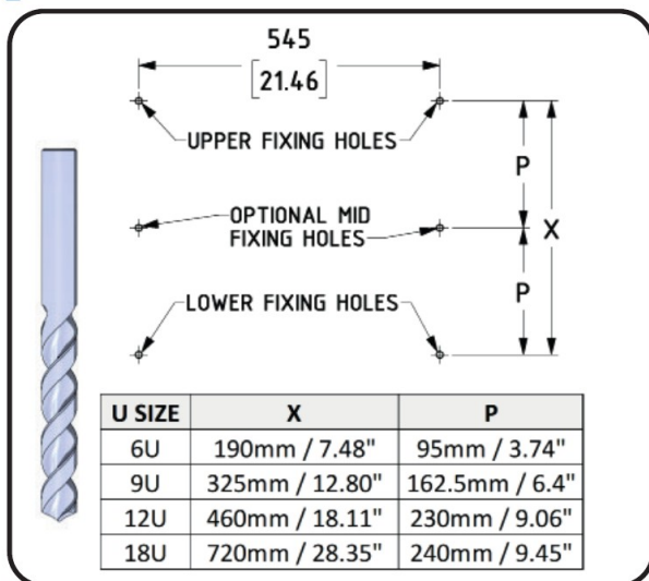
1. Drill Mounting Holes in Wall
