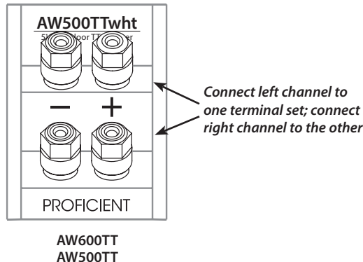
Diagram 1: Speaker Cable Terminals
