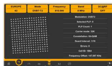
DVB-T2 Constellation
