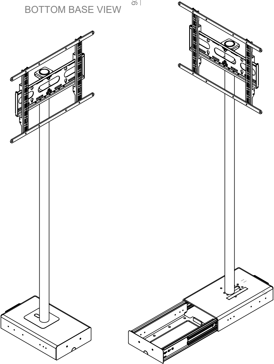
ISOMETRIC VIEW
