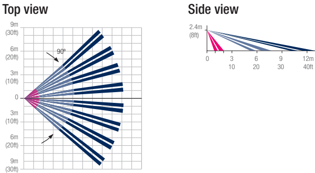
TOWER-20AM PG2 wide angle
